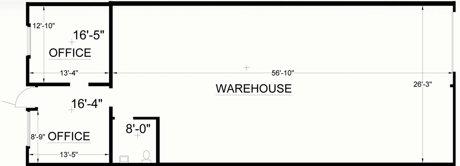
Current Floor Plan
